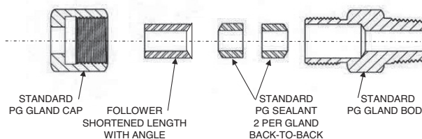
CONAX PG DOUBLE SEALANT GLAND FOR SEALING ON JACKETED CABLES
